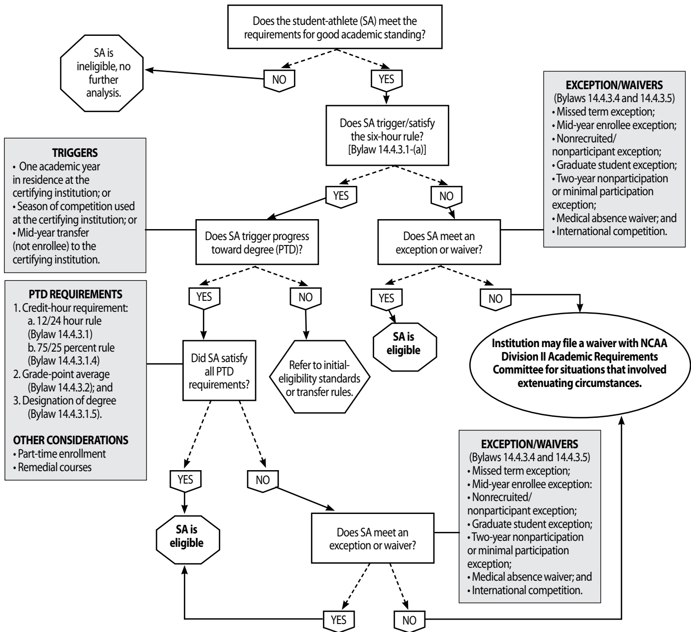
FIGURE 14-6 Progress-Toward-Degree Flowchart
